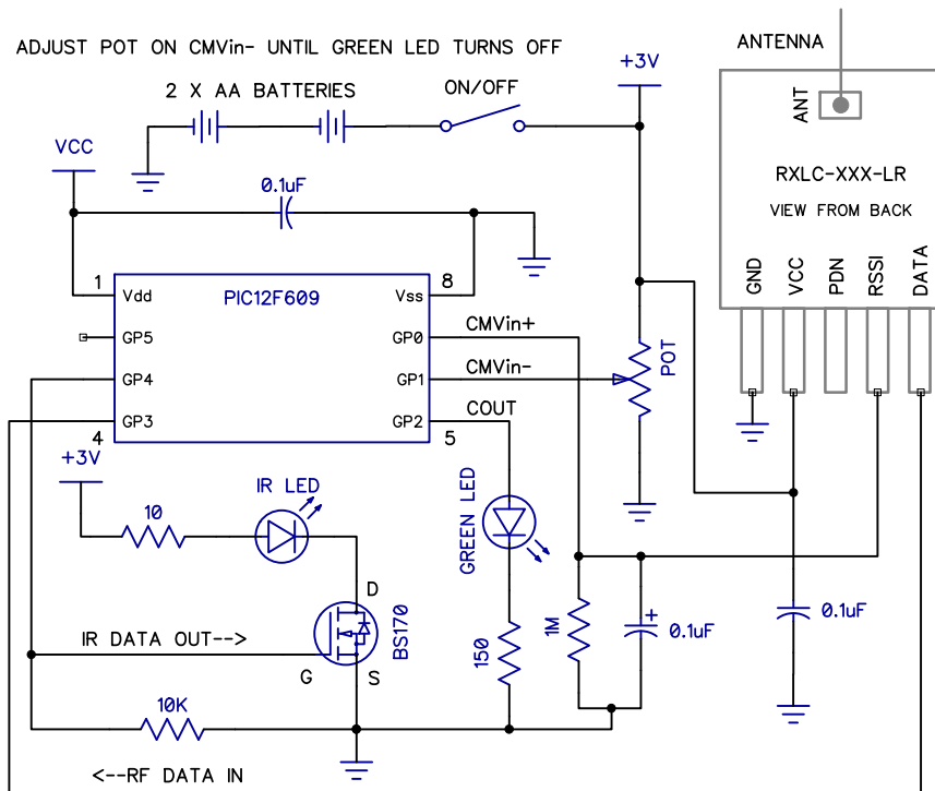
RF RECEIVER SECTION WITH INFRARED OUT
