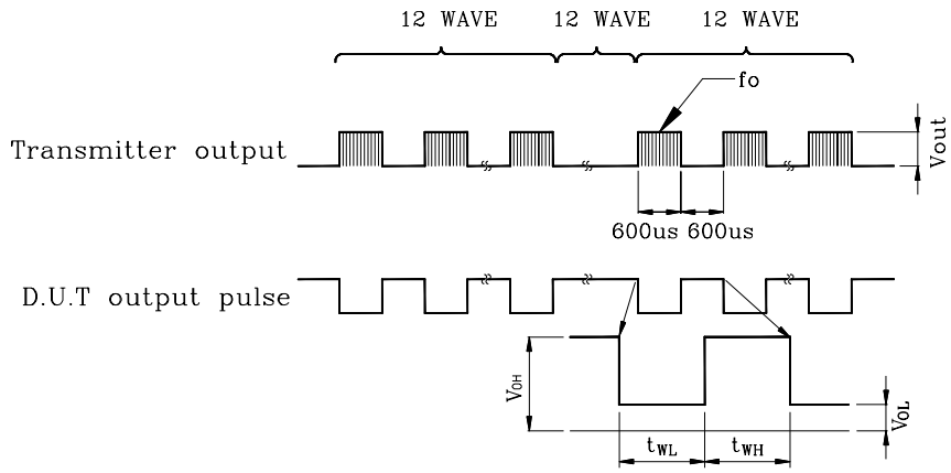
Fig. 4 Output pulse
