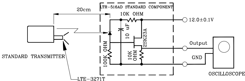
Fig. 3 Measuring method
